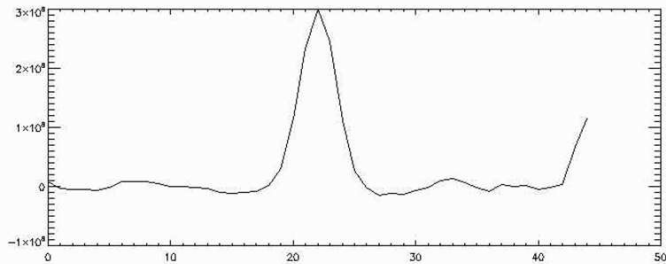
Figure 6. Long integration of the VEGA fringe signal with CLIMB used as group delay tracker. The vertical axis has just arbitrary units whereas the horizontal axis is a quantity proportional to the optical path difference.
